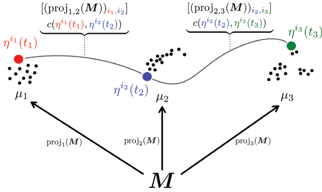
Fig. 4: The relationship between a transport plan M , its projections, and the transport cost C for n_s = 3 empirical distributions \{\mu_\sigma\}_{\sigma \in [n_s]} . Unimarginal projections equal the distributions, and for the three arbitrary colored points, [M_{i_1, i_2, i_3}] encodes the total probability mass transported, and [C_{i_1, i_2, i_3}] the per-unit cost thereof, along the grey-colored path therebetween. Similarly, the bimarginal projections of M and the pairwise cost c pertain to the pairwise sections of the path.
