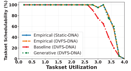
Fig. 8: Taskset Schedulability
